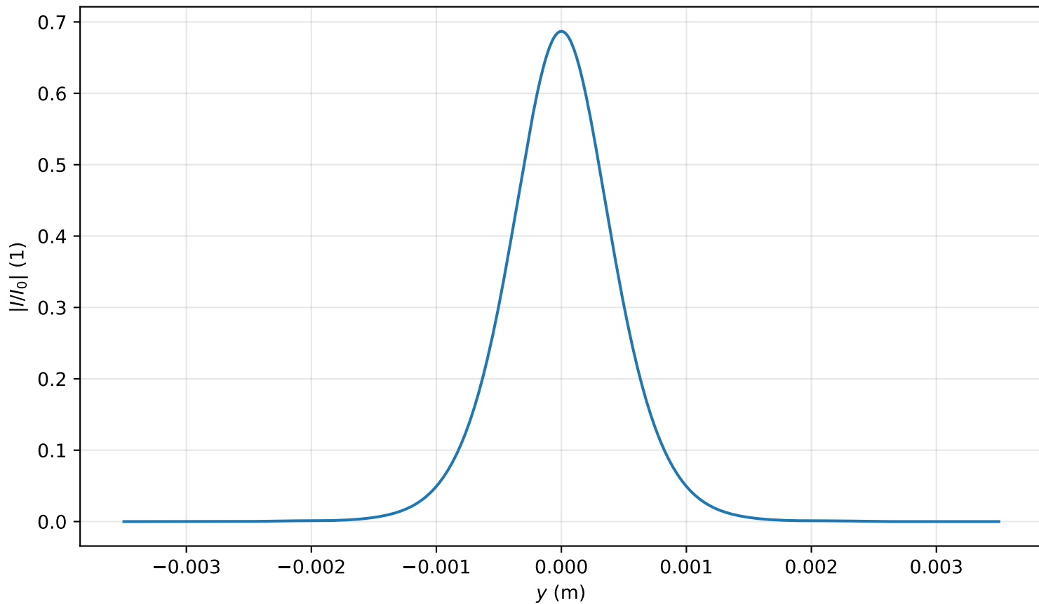
Intensity profile I(x = 0, y, z = 3.662)/I_0 , P_{in}=0.7P_{cr} , artificial time
